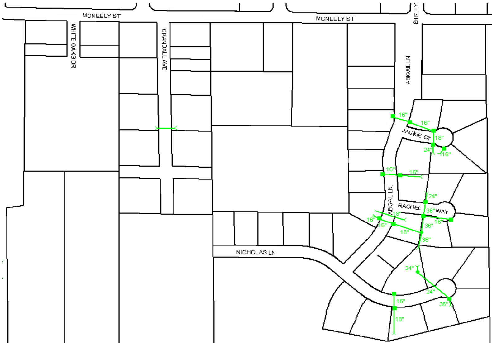
Overbrook Storm Water System
