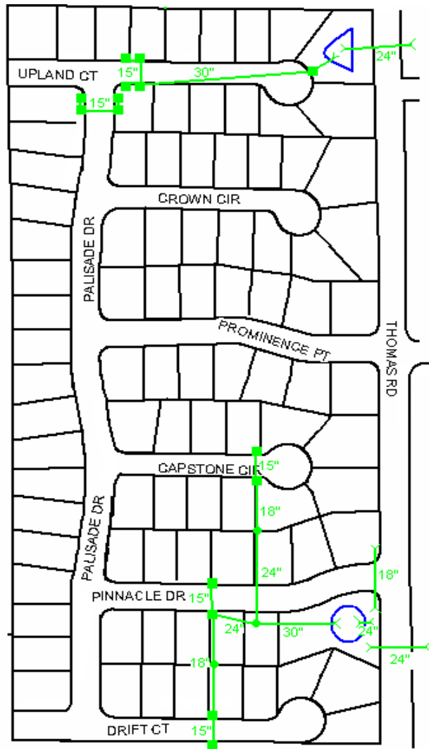
Prominence Point Storm Water System
